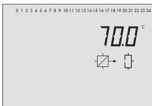
Flow sensor VF2, DHW circuit
